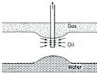
Fig. 11.15 Water and gas cone formation.
